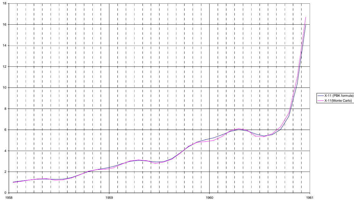
Figure 8: Box-Jenkins Airline Data Comparison of Formula and Monte Carlo Trend Revision Limits
