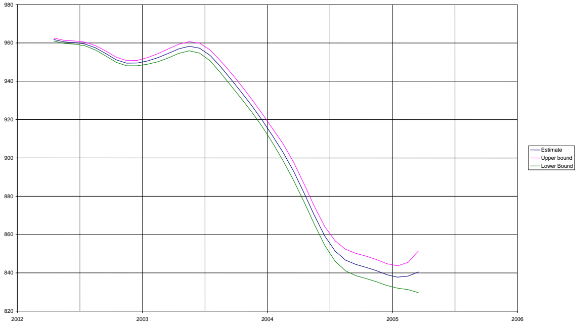
Figure 12: UK Claimant Count Unemployment Revision Limits for X-11 Trend (data to April 2005)
